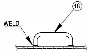
DETAIL OF GRAB HANDLE
