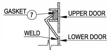
DETAIL OF DOUBLE HINGE
