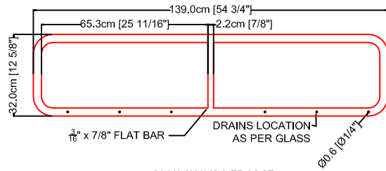
ALUMINUM FRAME SIZE AND DRAINS (OUTSIDE VIEW)
