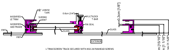
L TRIM/SCREEN TRACK SECURED WITH #10-24 PAN-HEAD SCREWS
