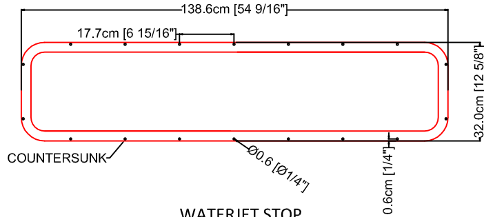
WATERJET STOP (AS VIEWED FROM INSIDE)
